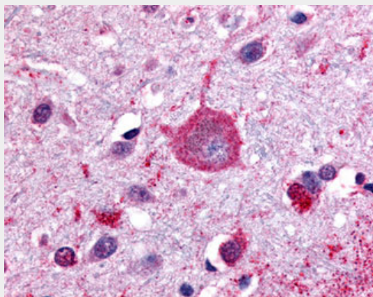
Anti-GPRC5B antibody ALS10731 IHC of human brain, cortex.
